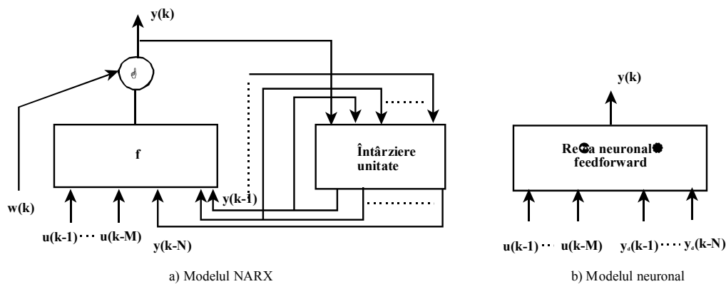
Fig. 5 The used model.
