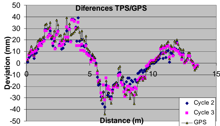
Fig. 5. The displacement measured by GPS and Total Station
