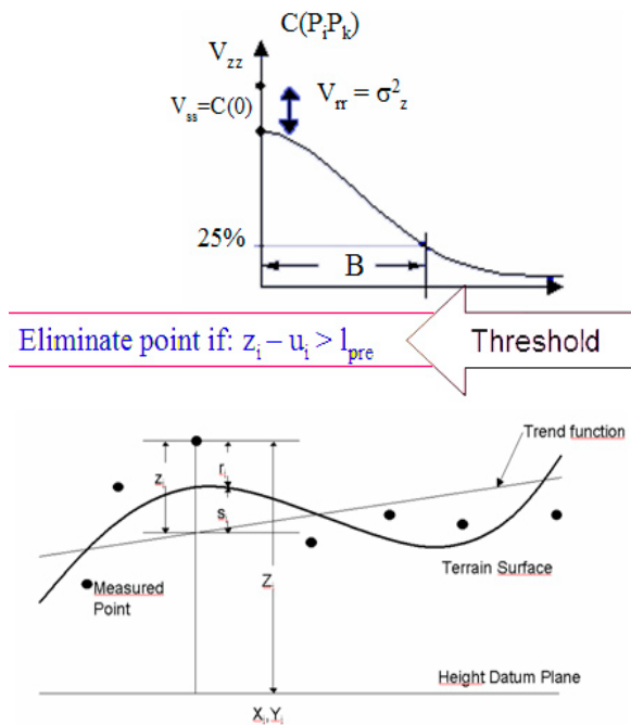
Fig. 4 Interpolation method [3]
